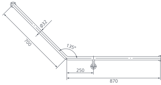
Front View (right hand)
