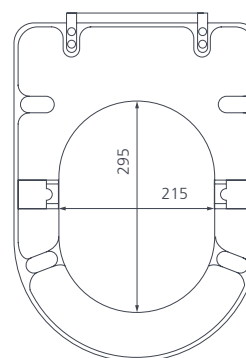
Seat view
