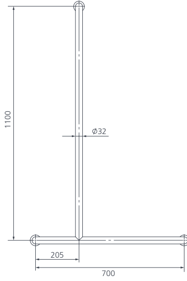
Front view (left hand)
