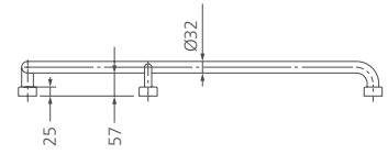
Side view (right hand)
