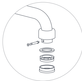
Concealed brass fixing mechanism
