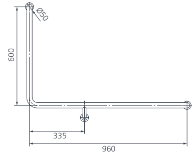
Front view (right hand)
