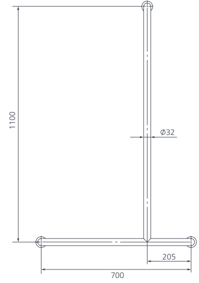
Front view (right hand)
