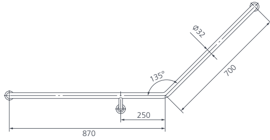
Front View (left hand)
